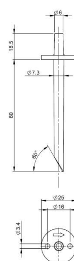
Duct connection for Climaset® 6555 / 6557
