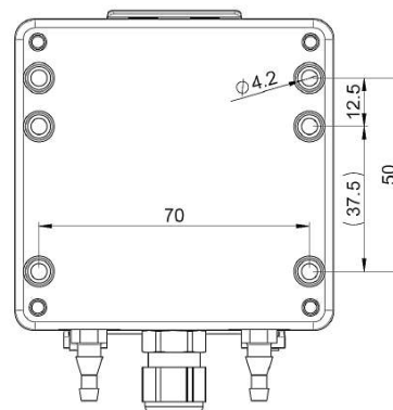
Drilling template
